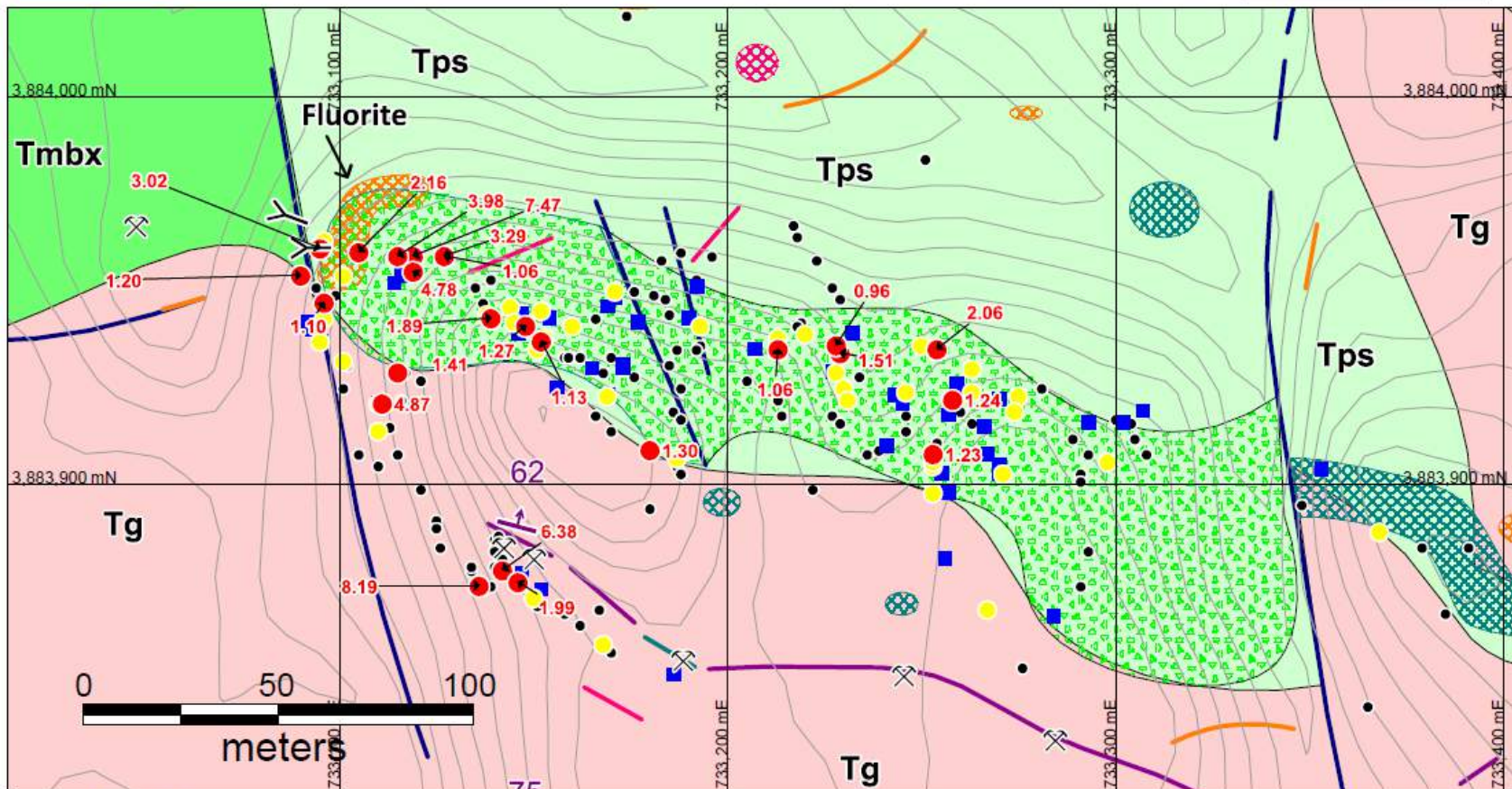
Fig. 1: Moss Property - West Oatman Area - Au in 2014 Rock Sampling
